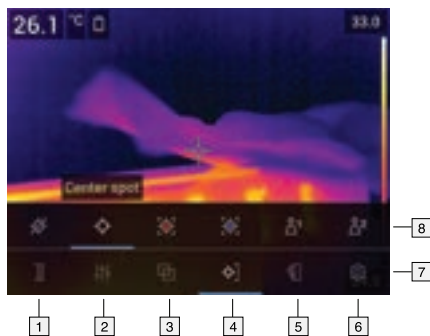
Figure 2.4 Menu system
