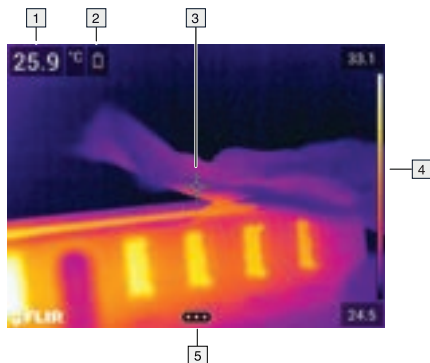
Figure 2.3 Screen elements
