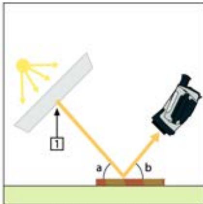
Figure 23.2 1 = Reflection source
