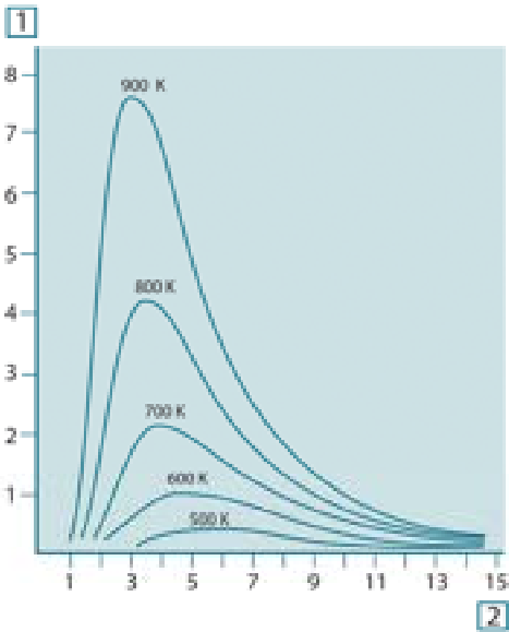
Figure 25.4 Blackbody spectral radiant emittance according to Planck's law, plotted for various absolute temperatures. 1: Spectral radiant emittance (W/cm² × 10³(μm)); 2: Wavelength (μm)
