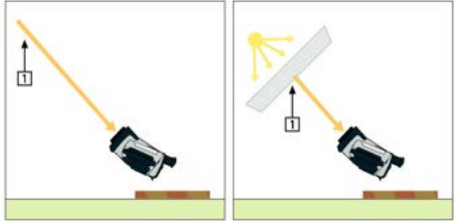
Figure 23.3 1 = Reflection source
