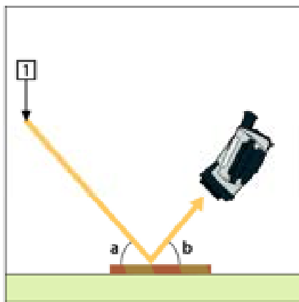
Figure 23.1 1 = Reflection source
